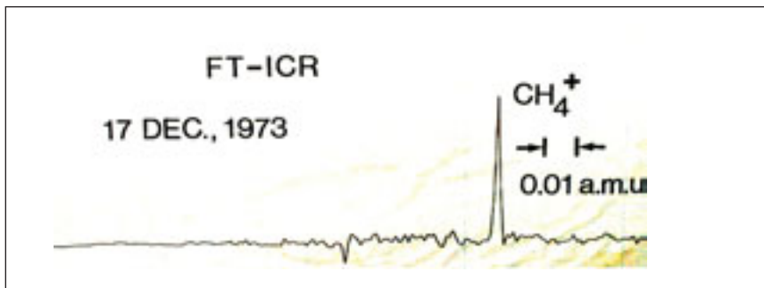
FIGURE 2: First FT-ICR mass spectrum, courtesy of Alan G. Marshall.
