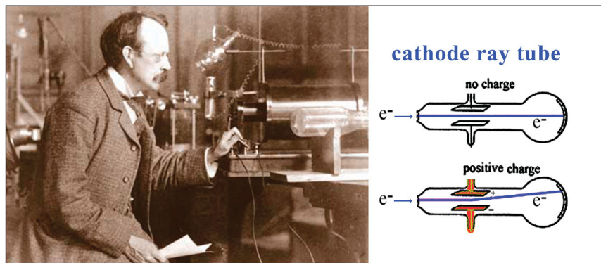
FIGURE 1: J. J. Thomson and a cathode ray tube used to perform some of the first m/z measurements. Deflection of the electron was observed once the electric field was turned on.
